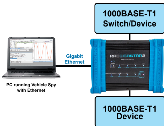
Using the RAD-Gigastar 2 as an active tap
